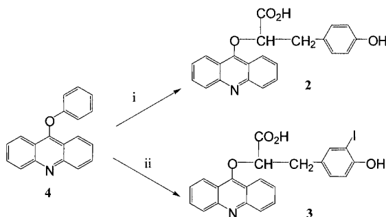
Scheme 3. Synthesis of compounds 2 and 3 : i) L-tyrosine, phenol, 100 °C, 98%; ii) L-3-Iodotyrosine, phenol, 100 °C, 93%
