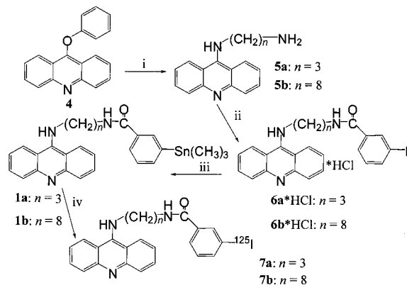
Scheme 1. i) \text{H}_2\text{N}(\text{CH}_2)_n\text{NH}_2 ( n = 3, 8 ), DMF, 100 °C. ii) 3-iodobenzoyl chloride, NaOH, \text{H}_2\text{O} , chloroform. iii) For 1a : \text{K}_2\text{CO}_3 , \text{Sn}_2(\text{CH}_3)_6 , \text{Pd}(\text{PPh}_3)_4 , DMF, 100 °C; for 1b : \text{K}_2\text{CO}_3 , \text{Sn}_2(\text{CH}_3)_6 , \text{PdCl}_2(\text{PPh}_3)_2 , 1,4-dioxane, 60 °C iv) [ 125 I]NaI, MeOH, CAT, 5 min
