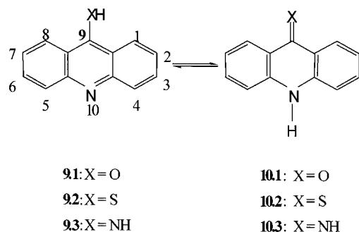
Scheme 2. Tautomerism in 9-substituted acridines
