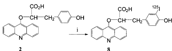
Scheme 4. Radioiodination of 2 : i) \text{Na}^{125}\text{I} , Chloramine-T
