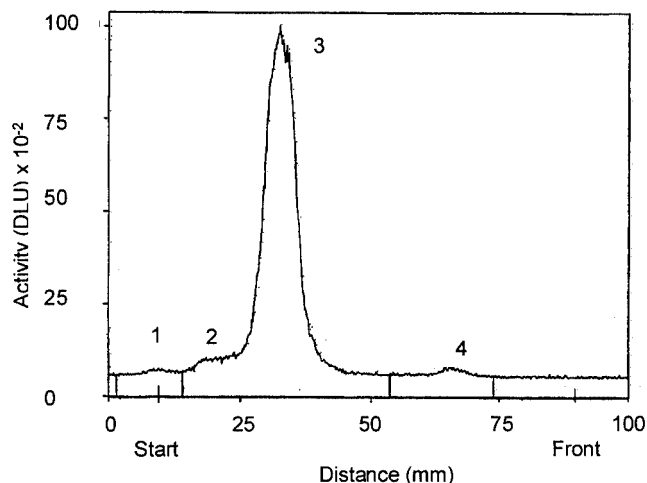
Figure 3. Radio iodination of 2-(acridin-9-ylamino)-3-(4-hydroxyphenyl)propionic acid ( 2 ); Merck silica gel 60 F 254 TLC aluminum sheets were used and the eluent was \text{CH}_2\text{Cl}_2/\text{CH}_3\text{OH} (4:1, v:v)
