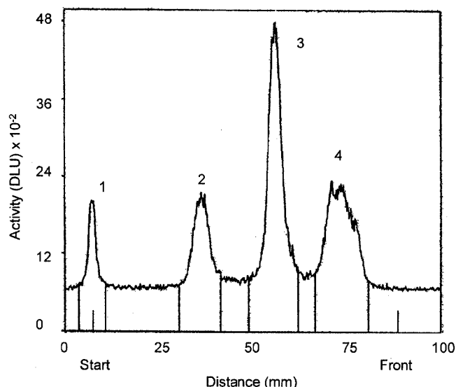
Figure 1. Radiochromatograms of a typical radioiodination with 1b ; Merck silica gel 60 F 254 TLC aluminum sheets were used and the eluent was CH 2 Cl 2 /CH 3 OH (3:1, v:v)
