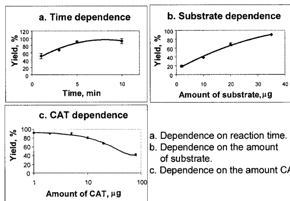
Figure 2. Dependence of radiochemical yields of 1b on different reaction conditions; experiments were performed in duplicate; error bars were calculated as maximal errors according to the formula: E_{r_{max}} = (Y_{max} - Y_{min})/2 ; total volume of reaction mixture was 70 µL; vessels were vortexed during reaction; the reaction was quenched with 20 µL sodium metabisulfite (3.3 mg/mL MeOH); sodium iodide (5 µL, 10 mg/mL MeOH) was added as carrier before analysis: a) 1b : 35 µg; CAT: 5 µg.; b) CAT: 5 µg, time: 5 min; c) 1b : 35 µg, time: 5 min
